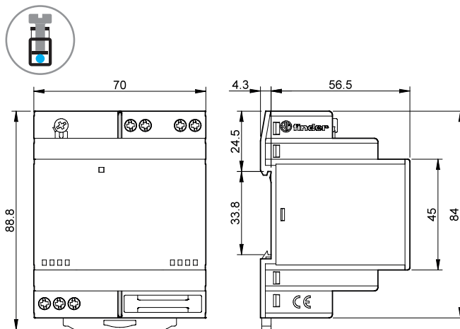
Typ 78.61 Screw terminal
