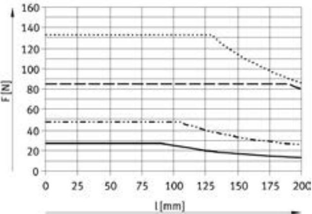
DFM-12 ... 25-GF, stroke 40 ... 100 mm
