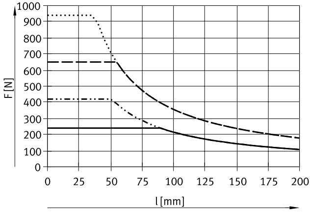
DFM-32 ... 63-GF, stroke up to 50 mm
