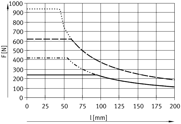
DFM-32 ... 63-GF, stroke 80 ... 100 mm
