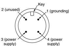
4-pin type
