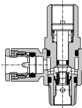
Meter-in type
