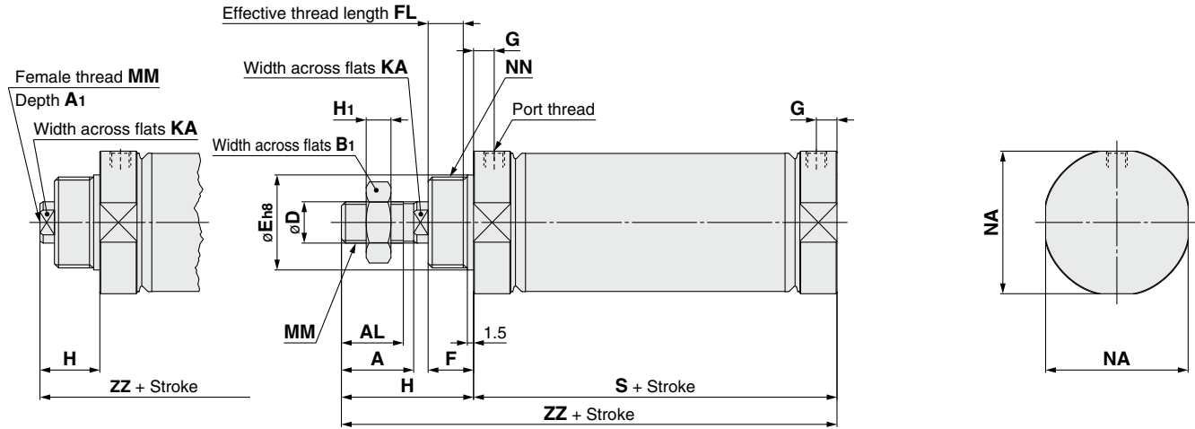
Female rod end
