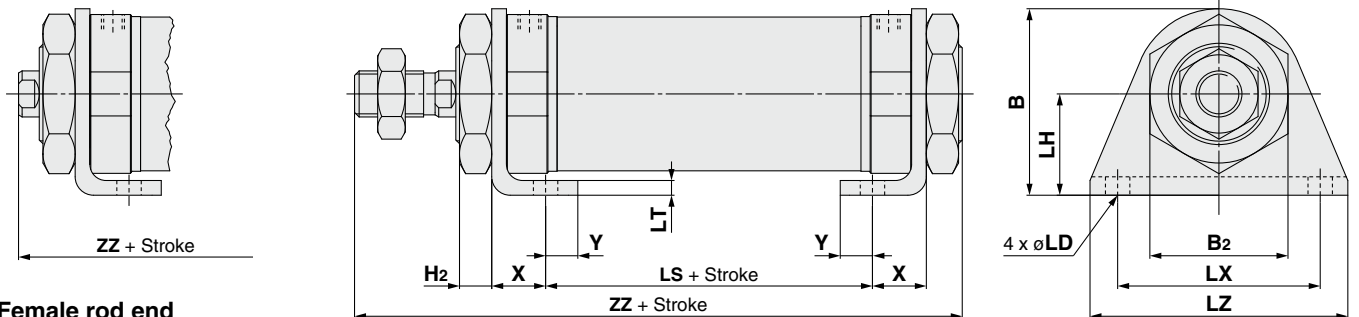
Female rod end
