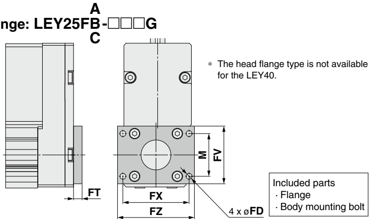
Rod/Head Flange [mm]
