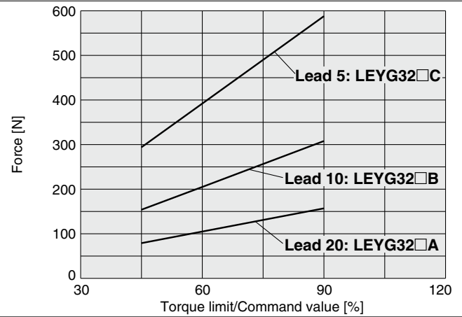
LEYG32□V7 (Motor mounting position: Parallel)
