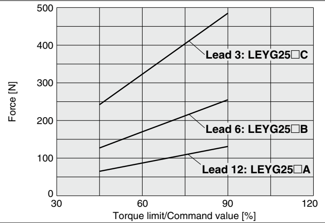
LEYG25□V6 (Motor mounting position: Parallel/In-line)
