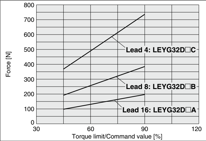
LEYG32DV7 (Motor mounting position: In-line)
