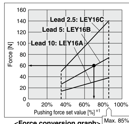
<Force conversion graph> (LEY16/Step motor)
